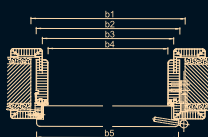
Horizontal cut panel (RF) Rebated single doors
