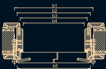
Horizontal cut panel (RF) Rebated double doors
